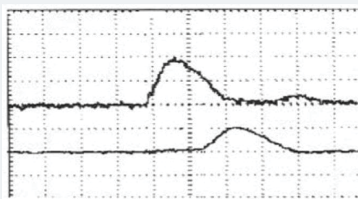
Figure 4: Oscillograms for the current through the initiating (upper trace) and control (bottom trace) wires. The timescale is 50 \text{ ns div}^{-1}
