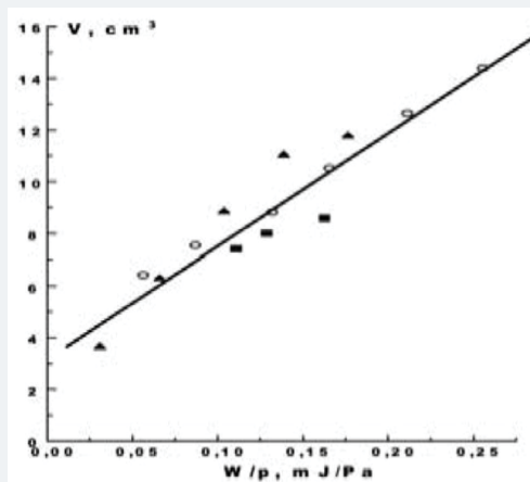
Figure 5: Dependence of volume V occupied by SIVD on W/p . Mixture: \text{SF}_6:\text{C}_2\text{H}_6=10:1 . I-p=5 \text{ Torr} ; A-p=30 \text{ Torr} ; and O-p=45 \text{ Torr}
