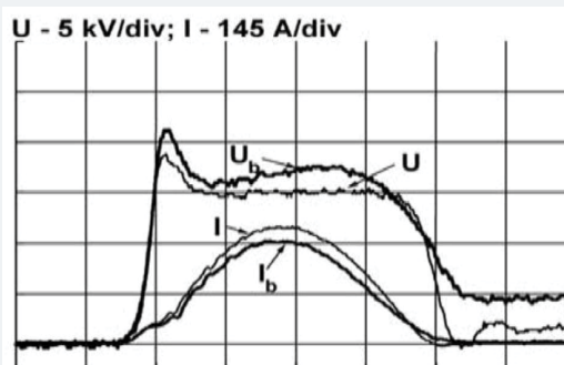
Figure 6: Experimental voltage and current oscillograms for bounded ( U_b, I_b ) and free ( U, I ) discharges. Timescale: 50\text{ns div}^{-1}
