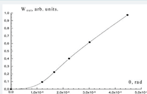
Figure 15: Angular distribution of the radiation energy in the far zone.
