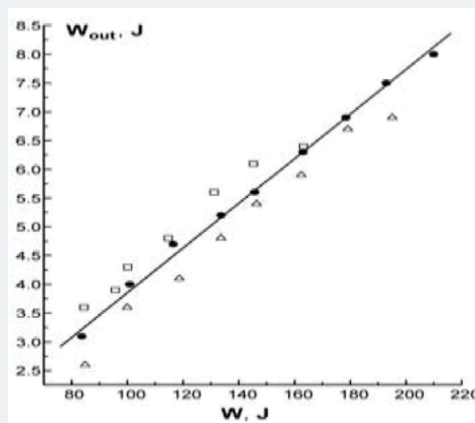
Figure 13: Dependences of the output laser energy ( W_{\text{out}} ) (generation on HF) on energy W deposited in the discharge plasma obtained for mixtures of \text{C}_2\text{H}_6:\text{SF}_6 with different component ratios: □-1:22, ●-1.5:22 and △-2:22.
