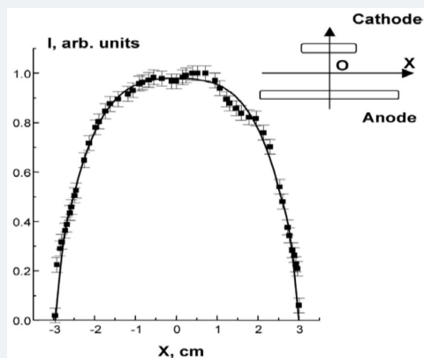
Figure 14: Plasma intensity distribution over the optic axis-contained plane placed in parallel to the electrode surfaces.
