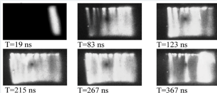
Figure 2: SIVD frames for different T -values.
