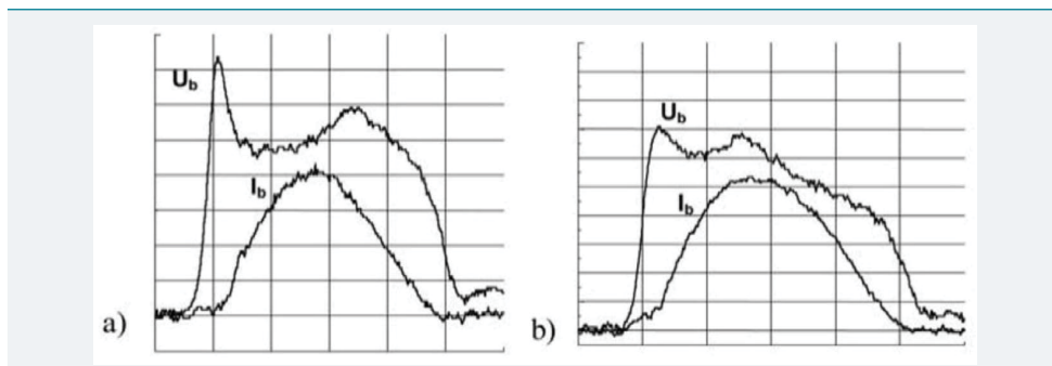
Figure 7: Current ( I_b ) and voltage ( U_b ) oscillograms for a bounded SIVD. Timescale: 50ns div -1 (a) -30 Torr C_3F_8 and (b) mixture: 15Torr C_2HCl_3 +3 Torr C_2H_6 .
