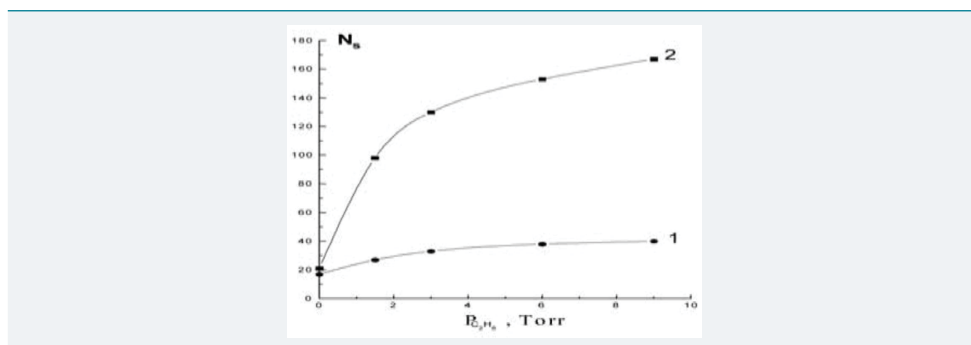
Figure 10: Dependences of the cathode spots number N_s on a partial pressure of C_2H_6 in SF_6-C_2H_6 mixture. SF_6 pressure p=30 Torr. 1–polished cathode and 2–cathode subjected to sandblasting.
