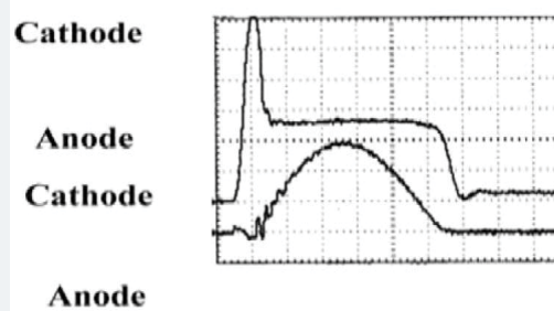
Figure 3: Typical oscillograms for the voltage (upper trace) and current (bottom trace). Timescale: 100 \text{ ns div}^{-1}
