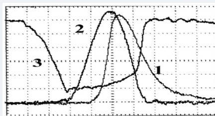
Figure 12: Typical oscillograms of laser pulse (1), current pulse (2) and voltage across the discharge gap (3) for the mixture 66 Torr \text{SF}_6 +6 Torr \text{C}_2\text{H}_6 . Scales: current—3Ka \text{div}^{-1} , voltage—10kV \text{div}^{-1} and time—100ns \text{div}^{-1} .
