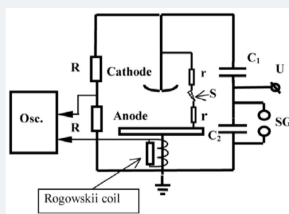
Figure 11: Electrical scheme of the non-chain HF (DF) laser.
