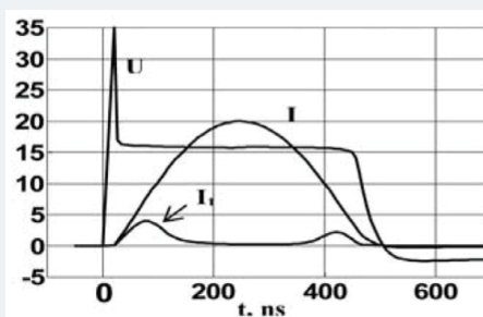
Figure 8: Oscillograms for voltage U and general current I , and the current through the first channel I_1 , scales: current—25A div -1 , voltage—5kV div -1 and time—200ns div -1 .
