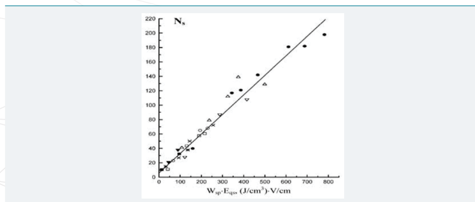
Figure 9: Dependence of the number of cathode spots N s on W sp ·E qs for the SF 6 : C 2 H 6 =10:1 mixture with d=6 cm and p=33.6 Torr (□), d=6 cm and p=16.8 Torr (■), d=4 cm and p=23.3 Torr (*), d=3 cm and p=23.3 Torr (▼), d=3 cm and p=33.6 Torr (○), d=3 cm and p=50.4 Torr (Δ), d=3 cm and p=67.2 Torr (◊), and d=2 cm and p=33.6 Torr (x).
