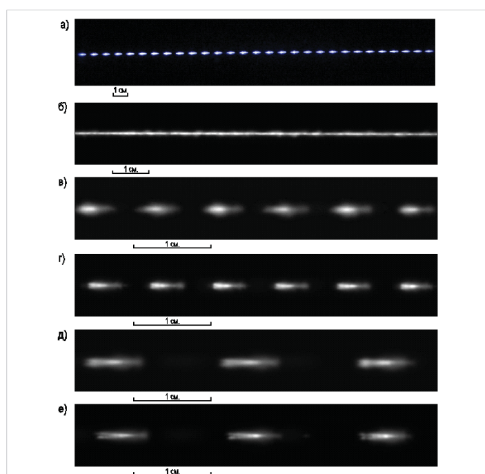
Figure 1: Time controlled evolution of trains in the space for F = 20 Hz, 50 cm/s and for F = 25 kHz, 250 cm/s correspondingly.
