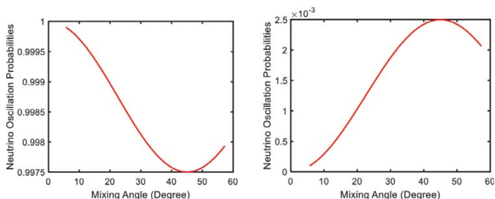
Figure 1: Two flavor neutrino oscillation probabilities.
