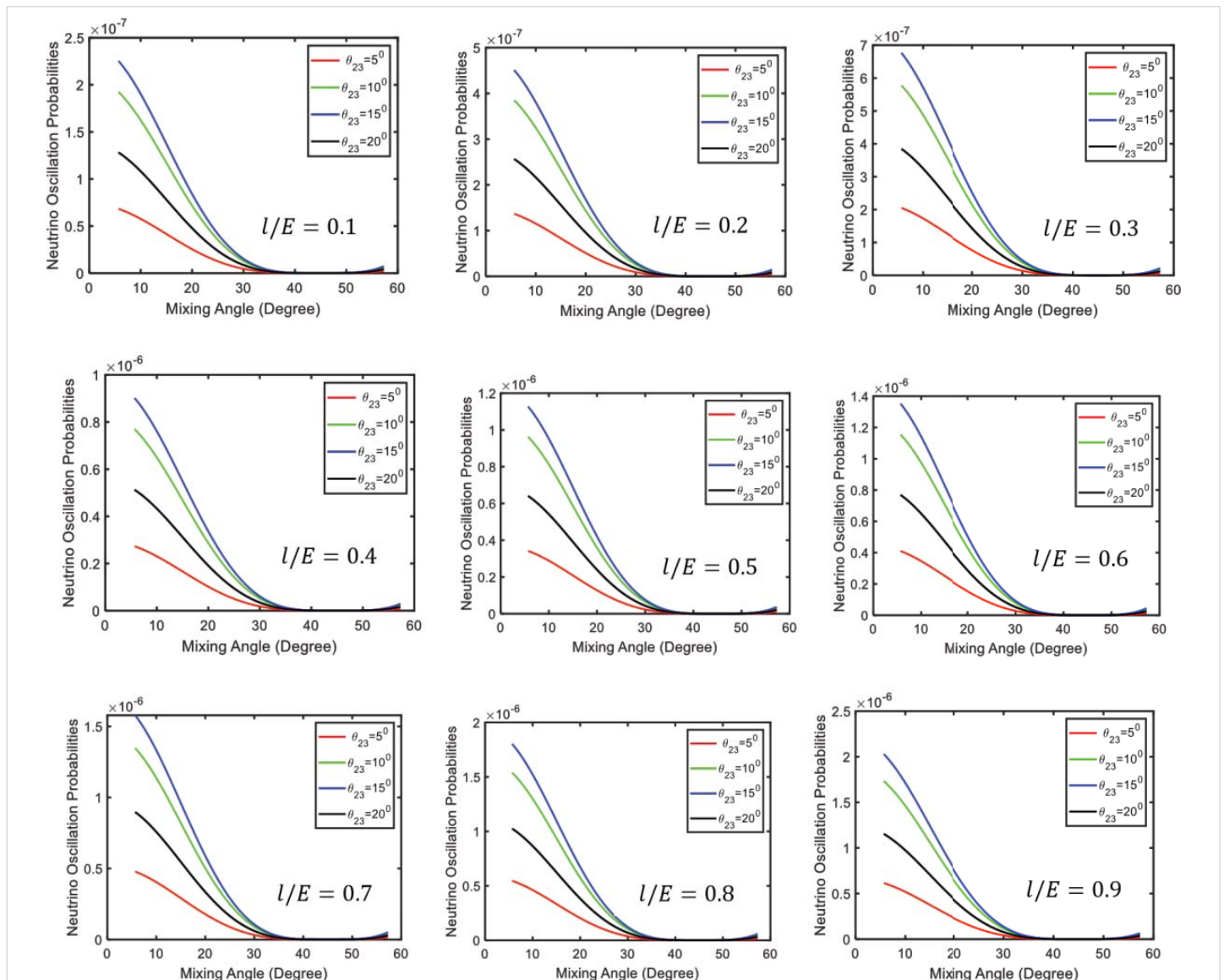
Figure 3: Three flavor neutrino oscillation probabilities \nu_\mu \rightarrow \nu_\tau
