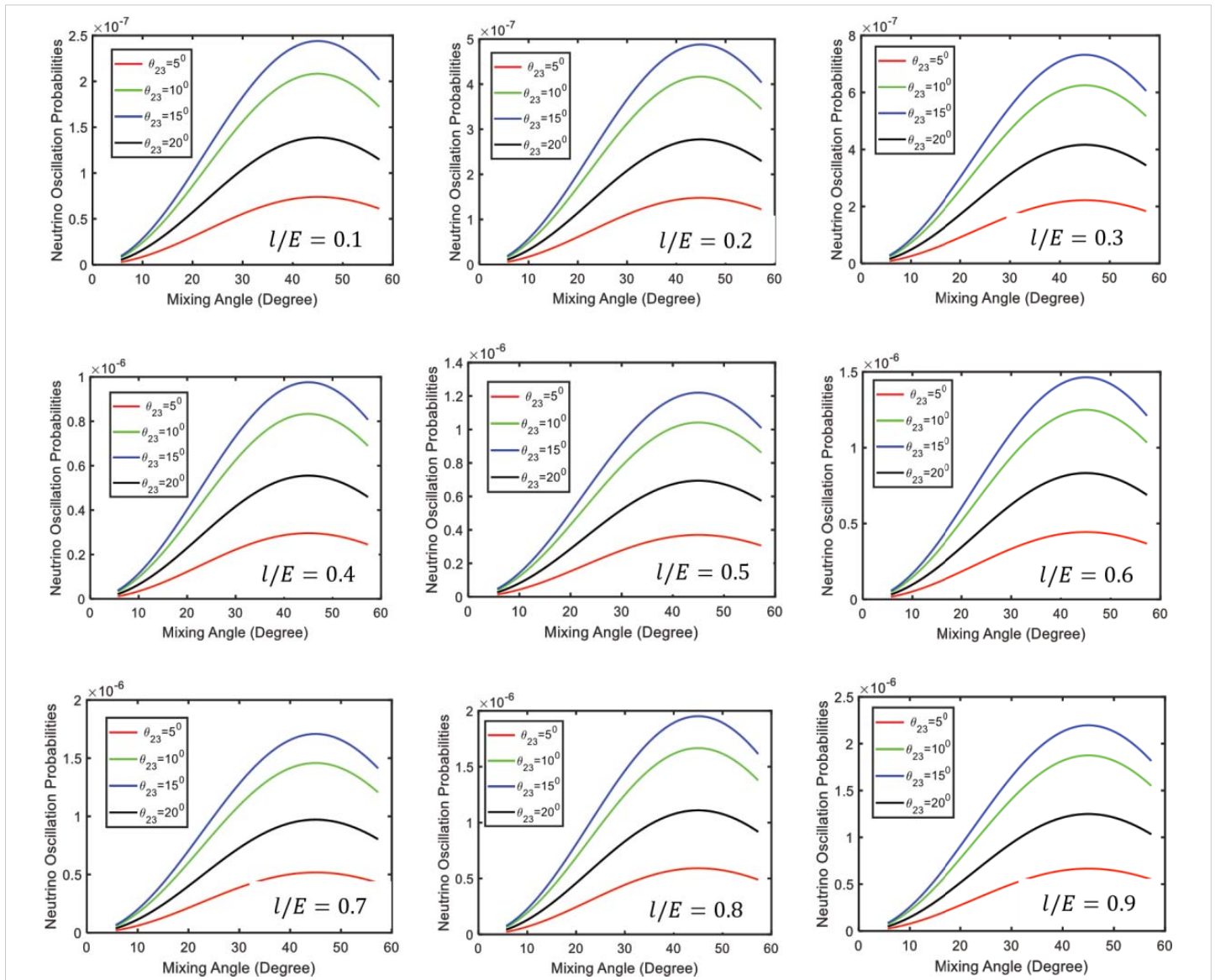
Figure 2: Three flavor neutrino oscillation probabilities \nu_e \rightarrow \nu_\mu
