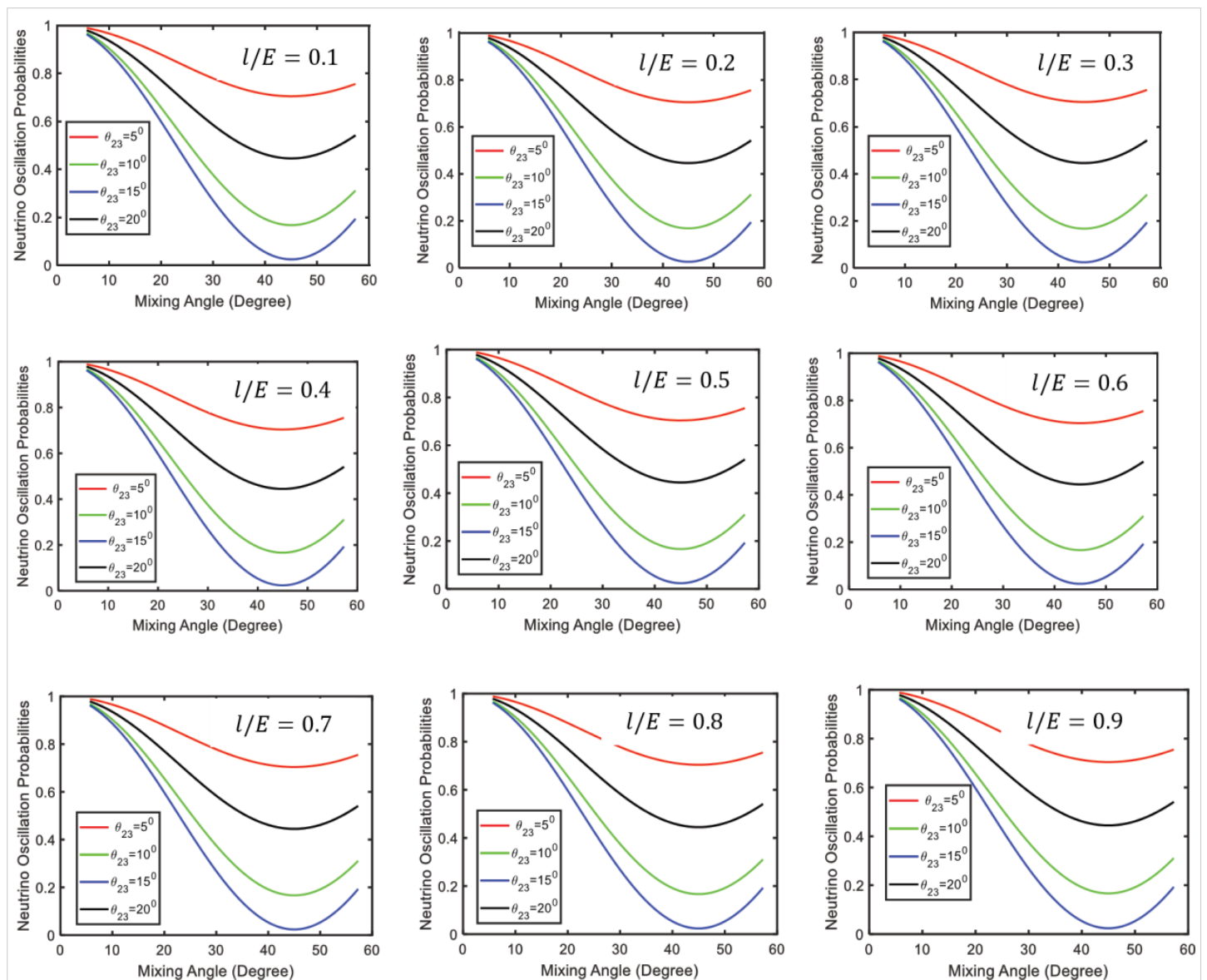
Figure 4: Three flavor neutrino oscillation probabilities \nu_\mu \rightarrow \nu_\tau
