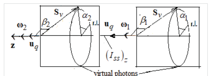
Figure 2: Schematic image of virtual photons created by positively charged quantum objects moving at velocity u_q . (I_{ss})_z is spin supercurrent along the axis z , \omega_1 and \omega_2 are precession frequencies, \alpha_1 and \alpha_2 are precession angles, \beta_1 and \beta_2 are deflection angles, S_v is spin, r.l. are reference lines.
