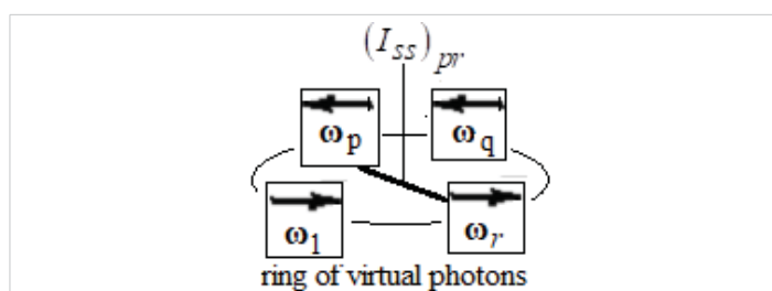
Figure 3: An example of the ring orientation of precession frequencies \omega_1, \omega_p, \omega_q, \dots, \omega_r of r virtual photons created by the quantum objects that constitute the substance of a cavity structure; (I_{ss})_{pr} is a spin supercurrent.
