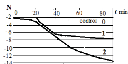
Figure 22: Dependence of CO_2 emission rate (in relative units N ) against time t . Curve 0 is the control measurement value without the use of magnetic vector potential. Curve 1 shows the measured values of CO_2 emission rate in case of “direct” action of the field-free magnetic vector potential. Curve 2 shows the measured values of CO_2 emission rate in case of “indirect” action of the field-free magnetic vector potential.
