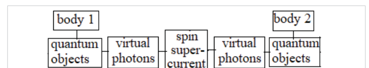
Figure 1: The schema of the interaction of two bodies (body 1 and body 2) by means of spin supercurrent emerging between virtual photons created by quantum objects of the bodies.
