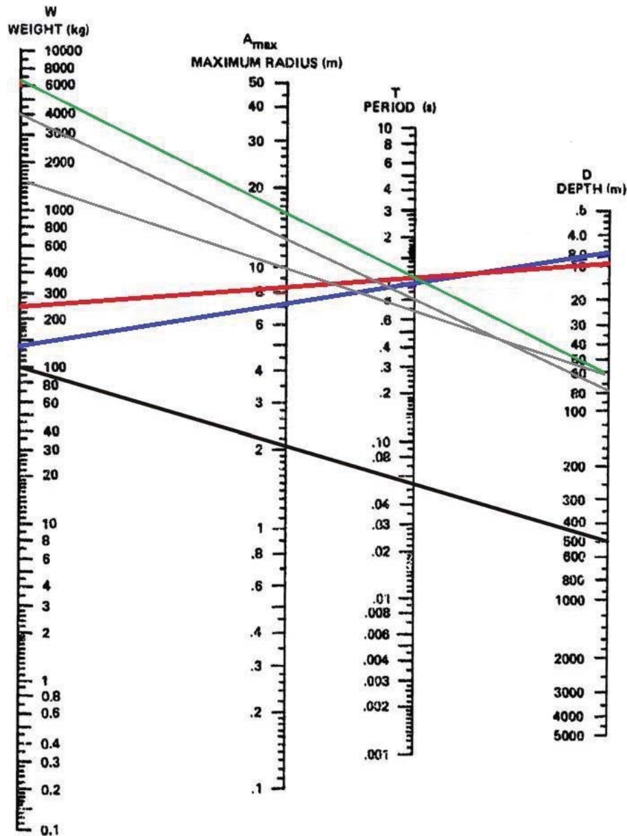
Figure 16: The nomograph of the first bubble pulse period, maximum bubble radius, and detonation depth for a gas bubble from underwater is modified adding more underwater explosion [20]. It is explosion examples. The thick blue, red, and black lines represent the detonation of 136 kg at a depth of around 8 m with a bubble pulse period of 0.988 s [1,3,4] and the detonation of 250 kg TNT at a depth of about 10 m with a bubble pulse period at 1.1 s [19] for the ROKS Cheonan Sinking and the detonation of 100 kg TNT at a depth of 500 m with a bubble pulse period of 0.05s and the maximum bubble radius of 2.033 m [20]. The thin green, brown, and gray lines indicate the detonation of 6759 kg TNT at a depth of 61 m ( M_L = 3.32 ) for the US Navy trial shock, 4020 kg TNT at a depth of 75 m [3] and 1500 kg TNT at a depth of 61 m for the Kursk submarine underwater explosion [3,24,37].
