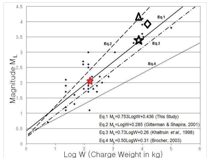
Figure 15: The reported magnitude for underwater and land detonations versus charge size. Empirical relations between local magnitude and underwater explosions from this study (Eq. 1) (solid line) [1], for Dead Sea underwater explosions with high salinity (Eq. 2) (dashed line) [35], the empirical upper limit magnitude of chemical land explosions in hard rock, for nuclear explosions (Eq. 3) (dotted and dashed line) [27] and coda magnitude of land explosions in California and Nevada, including most of coda duration magnitudes (Eq. 4) (dotted line) [36].
