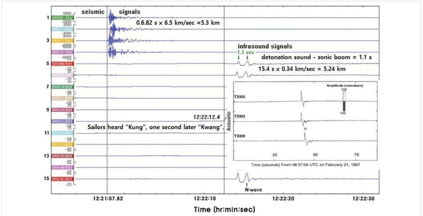
Figure 4: The infrasound records for the ROKS Cheonan Sinking on March 26, 2010. The inner figure shows seismic precursors to space shuttle fronts from the sound pressure N-wave recorded on 21 February 1997 as the STS-82 shuttle mission passed over the TXAR array [17].
