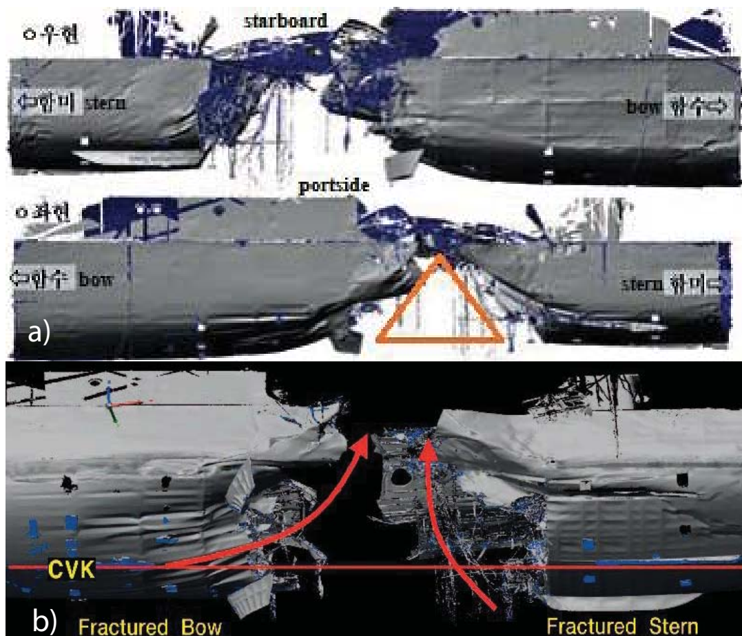
Figure 10: a) The split forms indicate that the split forms for starboard and portside fractures show an equilateral triangle-split form due to an explosion at the portside. b) The split ship is shown in a 3D laser scan image of the fractured bow and stern for the starboard side.
