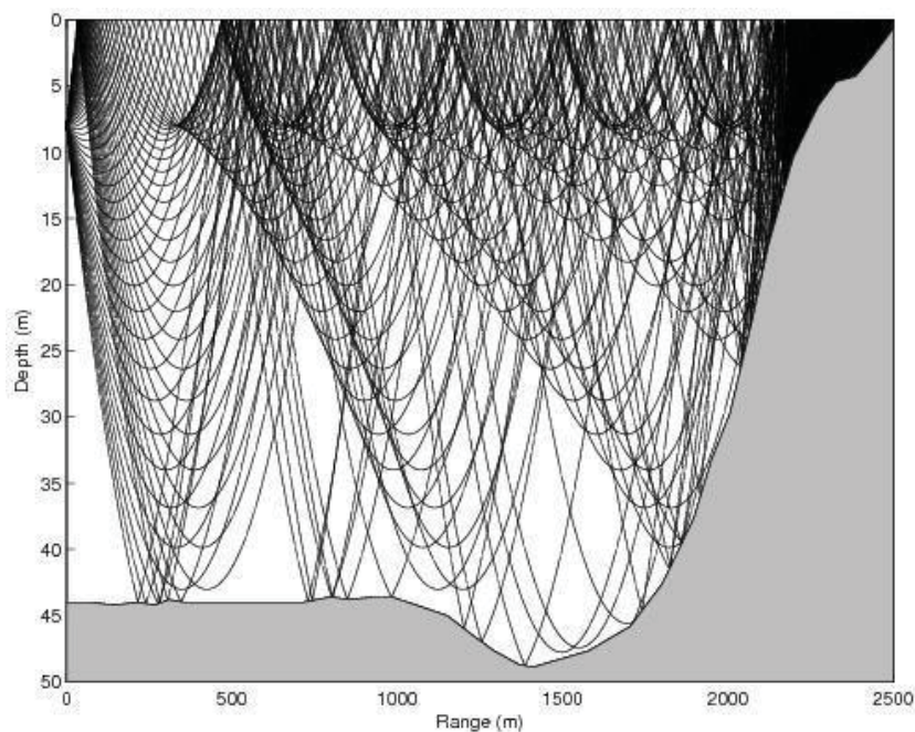
Figure 7: Ray-tracing based on hydroacoustic wave speed in the early spring season with a UWE source detonated at about 8 m offshore the Baengnyeong Island in the Yellow Sea. It exhibits shallow guided waves produced by total reflection of hydroacoustic waves from the free surface in the low-velocity layer at the subsurface and deep guided waves which are trapped by total reflection of hydroacoustic waves from the sea bottom [1-3].
