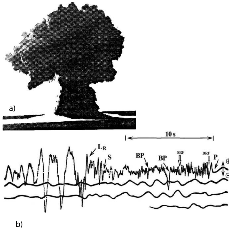
Figure 14: a) The Russian underwater explosion on October 3, 1961, showed a theoretical maximum height of about 2.2 km or at least greater than 1000 m according to the Swiadak experiment [20]. b) The vertical component seismogram represents the third Russian (USSR) underwater nuclear explosion which was conducted near Novaya Zemlya Island at 08:31:22.1 (GMT) on October 23, 1961 [30]. It was recorded in the town of Belushya 120 km away from the epicenter [30,31]. The bubble pulses (BP) with rarefaction (downward) distinctly appear on the seismogram.
