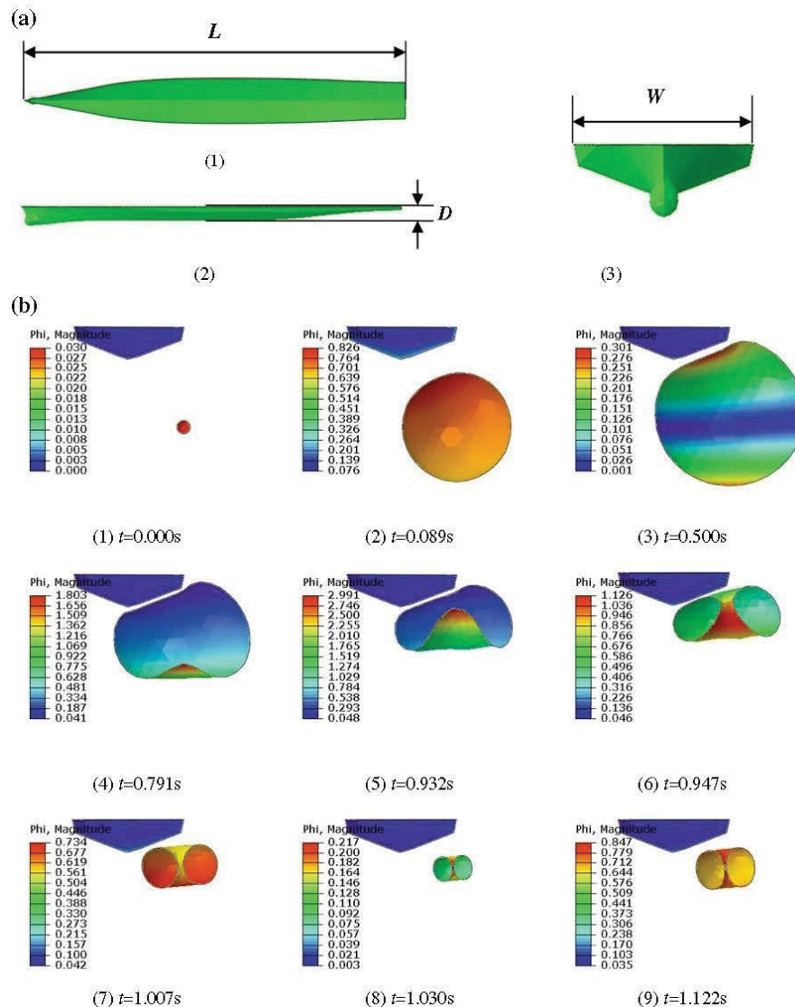
Figure 13: The behavior of 3D bubble shape simulation takes into account the interaction between the bubble and the ship’s hull based on the boundary element method (BEM). The color contour represents the magnitude of the velocity potential [13]. a. (1) bottom view ( L = 88 m) (2) side view ( D = 2.9 m) (3) front view ( W = 10 m). b. Bubble shape formation near ship’s hull: t = 0.000, 0.089, 0.500, 0.791, 0.932, 0.947, 1.007, 1.030, 1.122 s with 136-kg net explosive weight detonation at a depth of 8 and 5 m port side of the hull centerline. After a bubble pulse starts contracting, a toroidal bubble formation [9,10,12,13] at TB (0.791 s), just before a bubble pulse (BP) at 1.030 s and a bubble jet (BJ) occurs at around t = 1.007 s and the bubble gets a minimum at 1.030 s (BP) [2-4].
