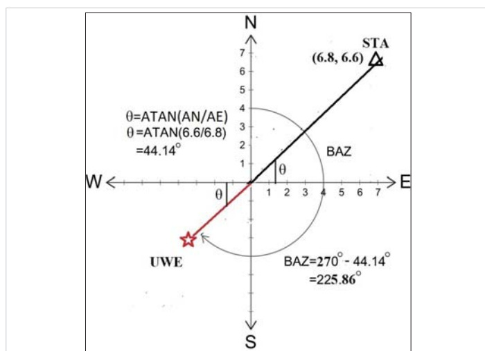
Figure 3: Determination of the direction of a site of the underwater explosion using the vector resultant of the first-arrival amplitudes (AN and AE) from two horizontal components of N-S and E-W and the positive motion of the first arrival on the vertical component. The positive first P-wave arrival on the vertical component means that the source is in the opposite to the station (+).
