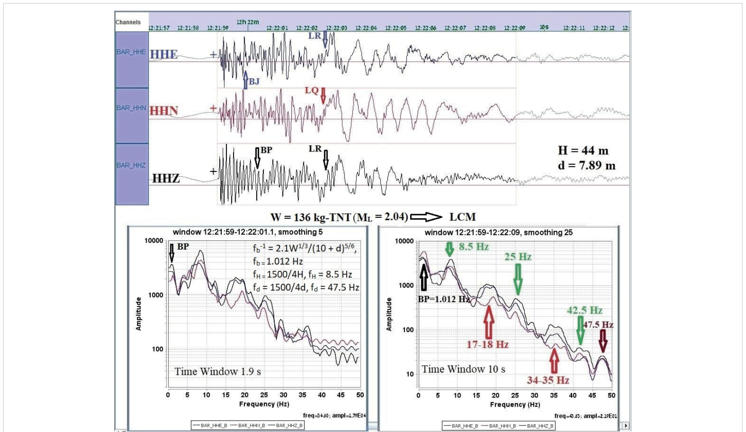
Figure 5: The positive (+) first motion of P-wave arrivals and the clear advent of a bubble pulse (BP) and a bubble jet (BJ) as well as Rayleigh (LR) and Love (LQ) waves in the time domain (upper) and spectral characteristic frequencies of 3-component spectra in the frequency domains (lower) at the BAR station comparing a short time window (1.9 s) with a long time window (10 s). The black arrows, red upward arrows, green downward arrows, and brown downward arrows indicate a bubble pulse frequency, reverberation frequencies from the bottom and reflection from the hull, and the reverberation frequency from the free surface, respectively.
