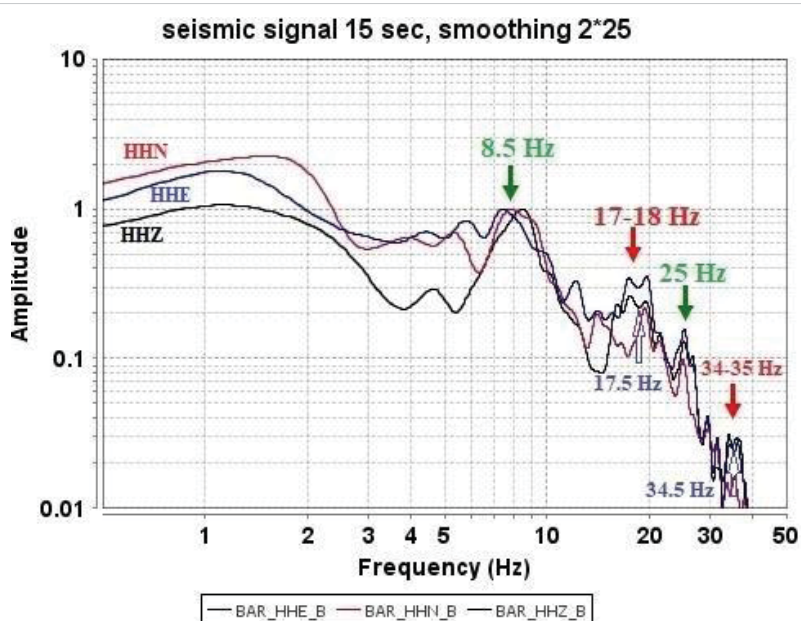
Figure 8: Smoothed normalized spectra of a seismic signal of time window 15 sec. The downward green arrows at 8.5 Hz and 25 Hz show reverberation frequencies from the seabed while the downward red arrows at 17 Hz - 18 Hz and 34-35 Hz reveal the reflected P-waves from the hull of the ship showing spectral nulls at 17.5 Hz and 34.5 Hz on the vertical and E-W (radial) components.
