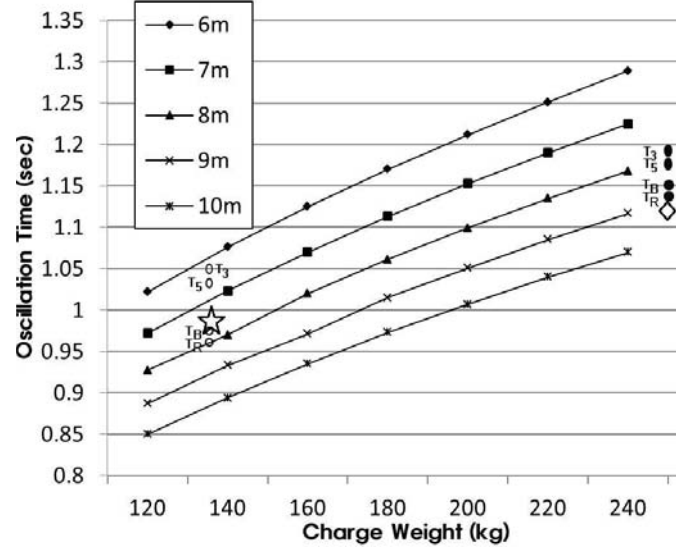
Figure 12: The relationships of the charge weights versus bubble pulse periods in the free surface. Distribution of possible bubble pulse periods by analytical solution [21] with Rayleigh-Willis equation (TR), BEM (TB), 3D simulation (T3, T5) for 136 kg net explosive weight (open ellipse) at a depth of 8 m at 3 m and 5 m port side of the hull centerline and for 250 kg net explosive weight (closed ellipse) at a depth of 9 m at 3 m and 5 m port side of the hull centerline [3,4].
