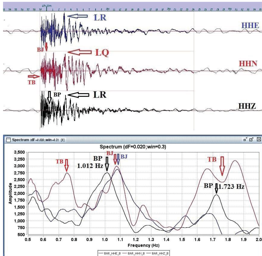
Figure 6: 3-component seismograms and high-resolution spectra for the ROKS Cheonan Sinking underwater explosion at BAR station. The characteristic motions of an underwater explosion (BP, BJ, and TB) are clearly shown on the 3-component (N-S, E-W, and Z) spectra. It is very remarkable to observe a toroidal bubble (TB) deformation which is followed by a bubble jet (BJ) immediately before a bubble pulse (BP) in the time domain as well as in the frequency domain. It is also possible to observe a series of clear modulations of bubble pulse at 1.012 Hz (first bubble pulse) and at 1.723 Hz (second bubble pulse) in the spectra.
