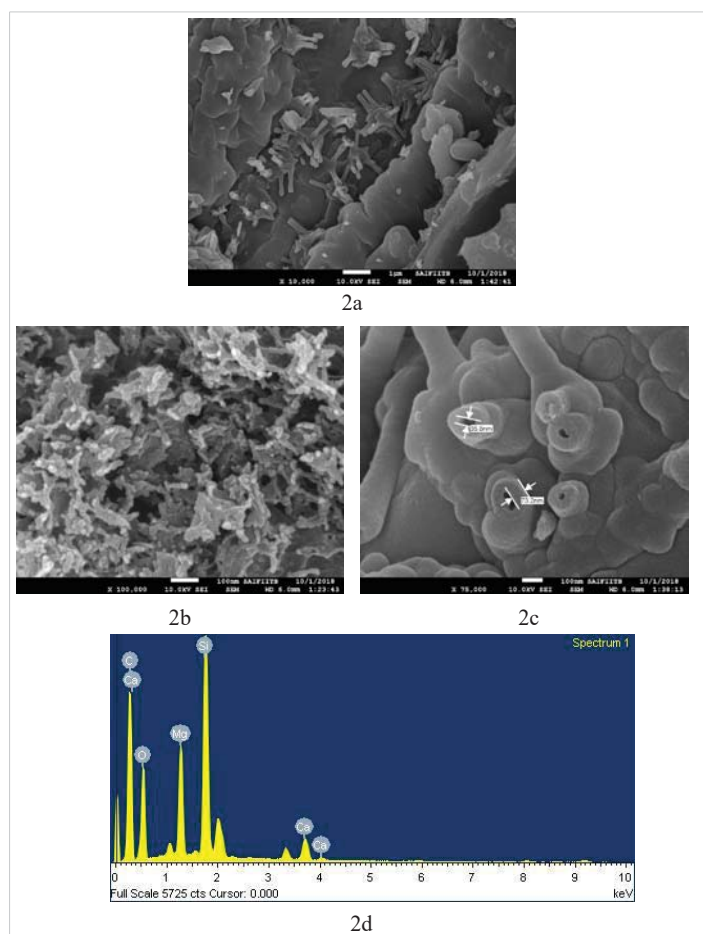
Figure 2: SEM image of 2a) As Grown CNFs; 2b) and 2c) Shape and size of CNFs purified with 50% Conc. HCl and HNO 3 ; 2d) SEM EDAX spectra of CNFs.
