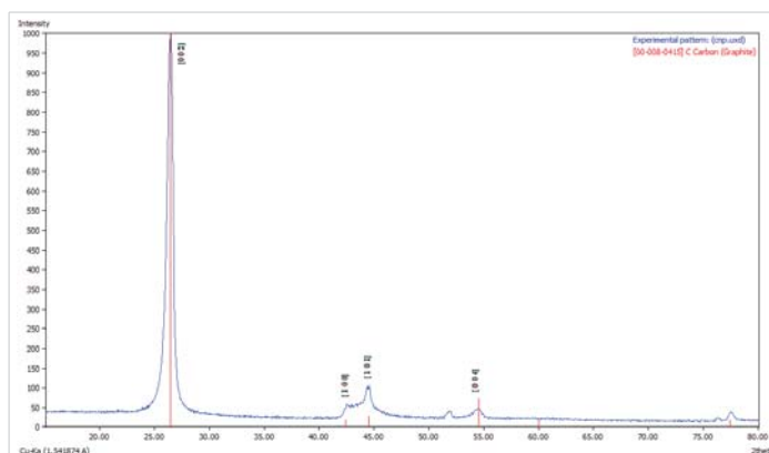
Figure 3b: XRD Spectra of Purified CNFs with 50% Conc. HCl and HNO 3 acids.
