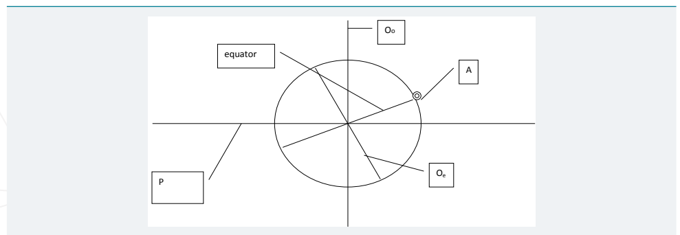
Figure 2: Flow chart of tides. P - lateral projection of the plane of the earth torsion. O_0 is the axis of rotation of the Earth's torsion bar. O_e is the axis of Earth's rotation. Point A crosses the plane of the earth torsion twice a day.
