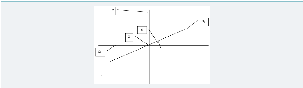
Figure 1: Cross section of the solar system. O_s - lateral projection of the orbit of the etheric solar torsion O_p - lateral projection of the planet's orbit Z - axis of rotation of the torsion bar O - projection of the line of intersection of the orbit of planets with a gravitational orbit
